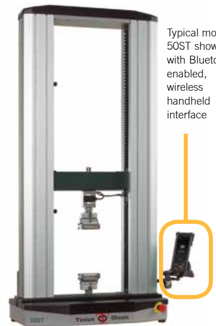
Model 50ST - 50 kN (5,000 kg/11,000 lbf)
